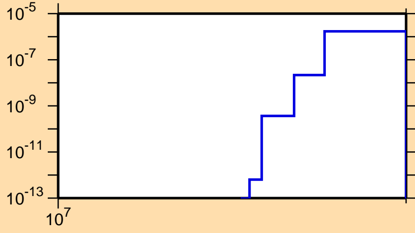
\sigma vs. E for ^{159}\text{Eu}(n,nt)
