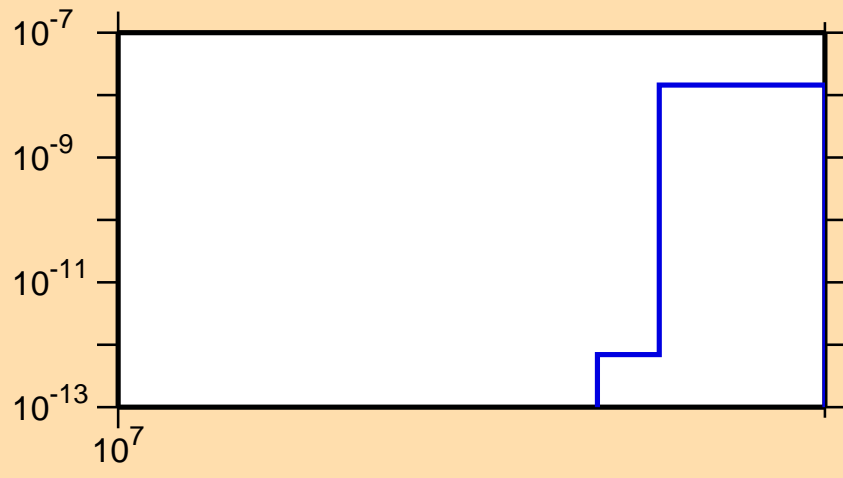
\sigma vs. E for ^{159}\text{Eu}(n,2np)
