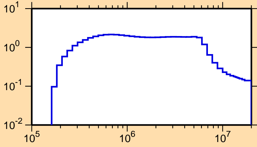
\sigma vs. E for ^{160}\text{Eu}(n,n\text{cont.})
