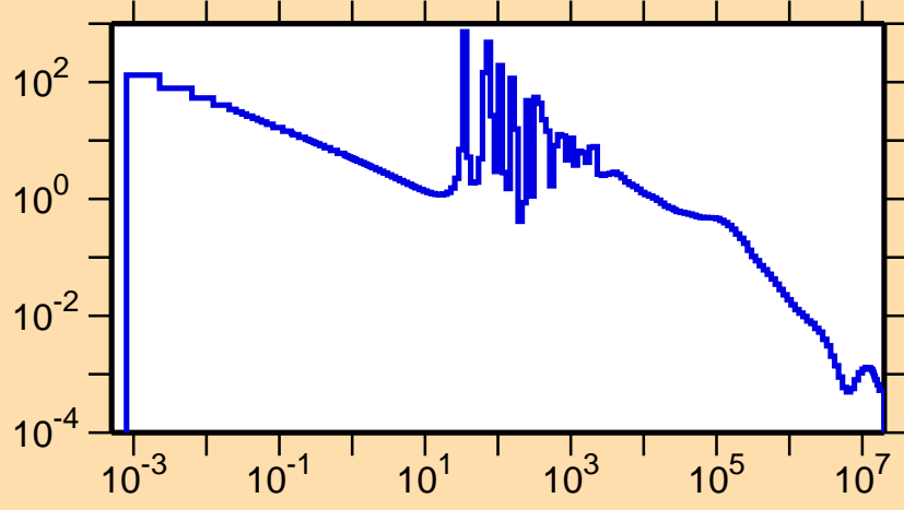
\sigma vs. E for ^{160}\text{Eu}(n,\gamma)
