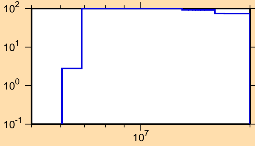
\Delta\sigma/\sigma vs. E for ^{161}\text{Eu}(n,p)
