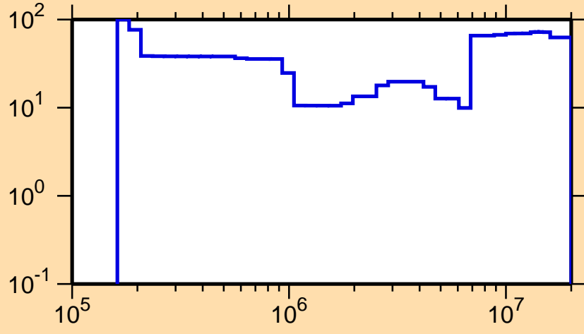
\Delta\sigma/\sigma vs. E for ^{161}\text{Eu}(n,\text{inel.})
