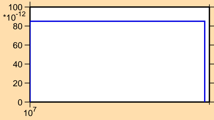
\sigma vs. E for ^{161}\text{Eu}(n,2np)
