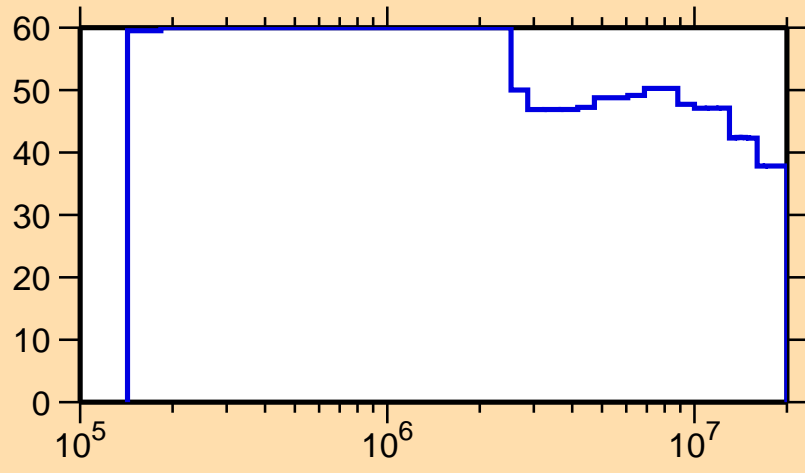
\Delta\sigma/\sigma vs. E for ^{162}\text{Eu}(n,n_1)
