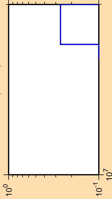
\Delta\sigma/\sigma vs. E for ^{162}\text{Eu}(n,3n\alpha)
