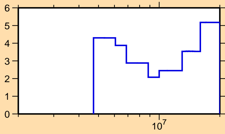
\Delta\sigma/\sigma vs. E for ^{162}\text{Eu}(n,\text{nonel.})
