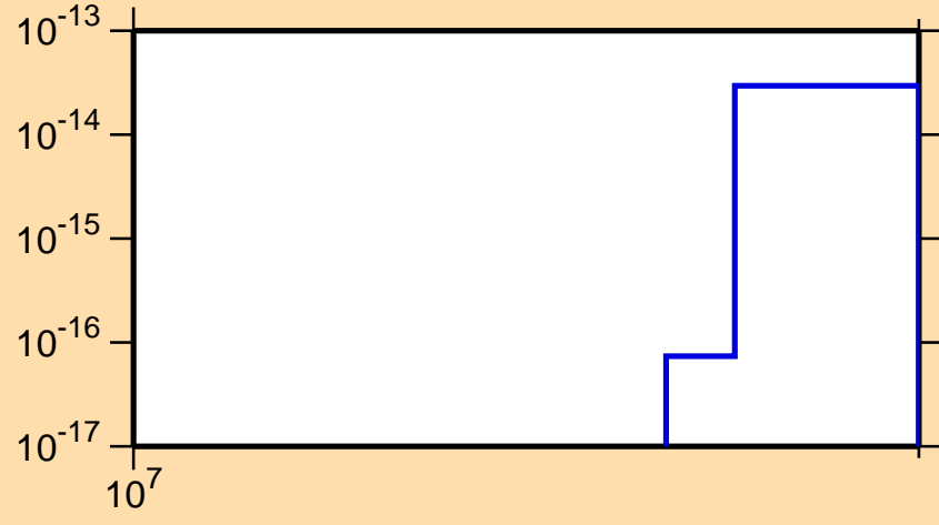
\sigma vs. E for ^{162}\text{Eu}(n,3n\alpha)
