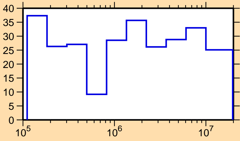
\Delta\sigma/\sigma vs. E for ^{162}\text{Eu}(n, el.)
