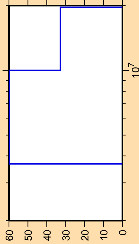
\Delta\sigma/\sigma vs. E for ^{162}\text{Eu}(n,2n)
