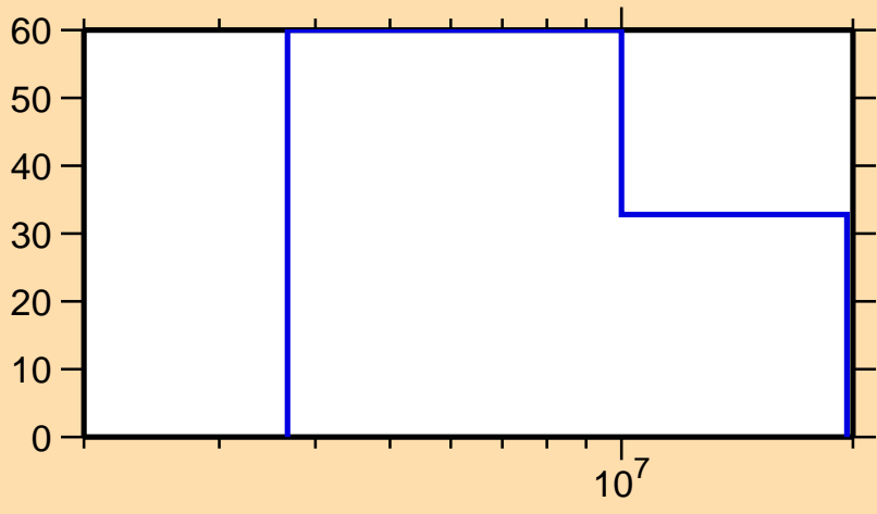
\Delta\sigma/\sigma vs. E for ^{162}\text{Eu}(n,2n)
