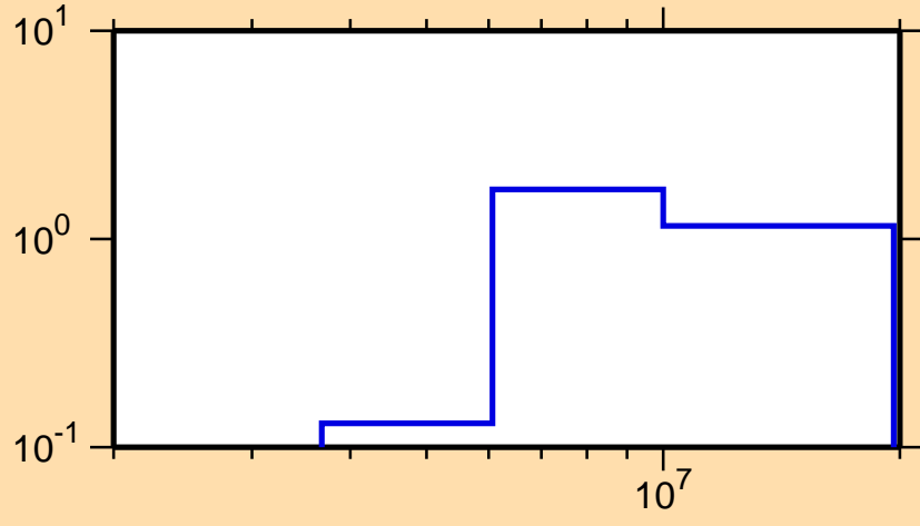
\sigma vs. E for ^{162}\text{Eu}(n,2n)
