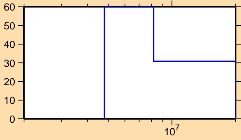
\Delta\sigma/\sigma vs. E for ^{162}\text{Eu}(n,2n)
