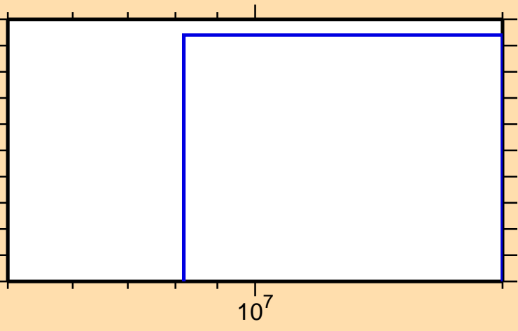
\sigma vs. E for ^{162}\text{Eu}(n,np)
