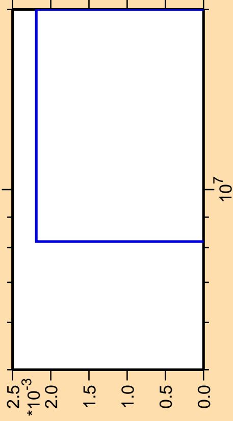
\Delta\sigma/\sigma vs. E for ^{162}\text{Eu}(n,3n\alpha)
