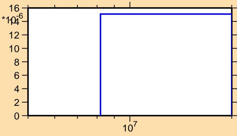
\sigma vs. E for ^{162}\text{Eu}(n,t)
