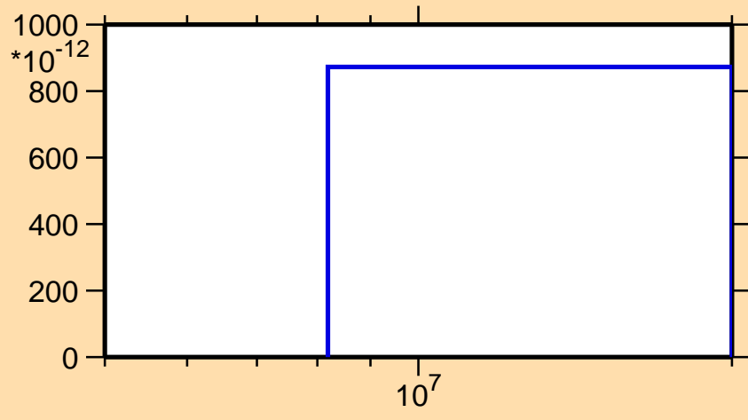
\sigma vs. E for ^{162}\text{Eu}(n,2n\alpha)
