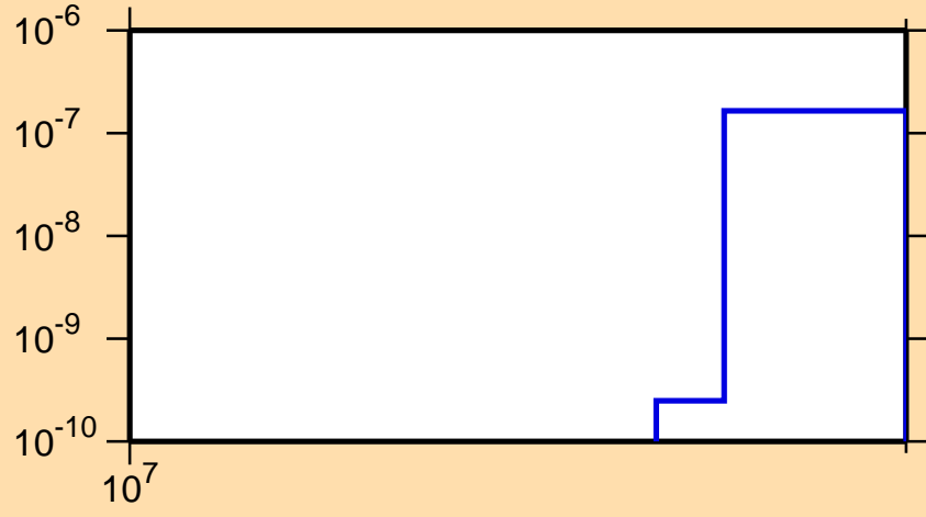
\sigma vs. E for ^{163}\text{Eu}(n,nd)
