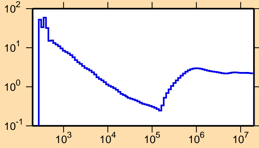
\sigma vs. E for ^{163}\text{Eu}(n,\text{nonel.})
