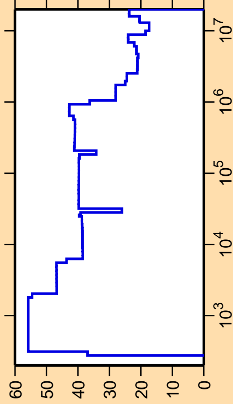
\Delta\sigma/\sigma vs. E for ^{163}\text{Eu}(n,\text{nonel.})
