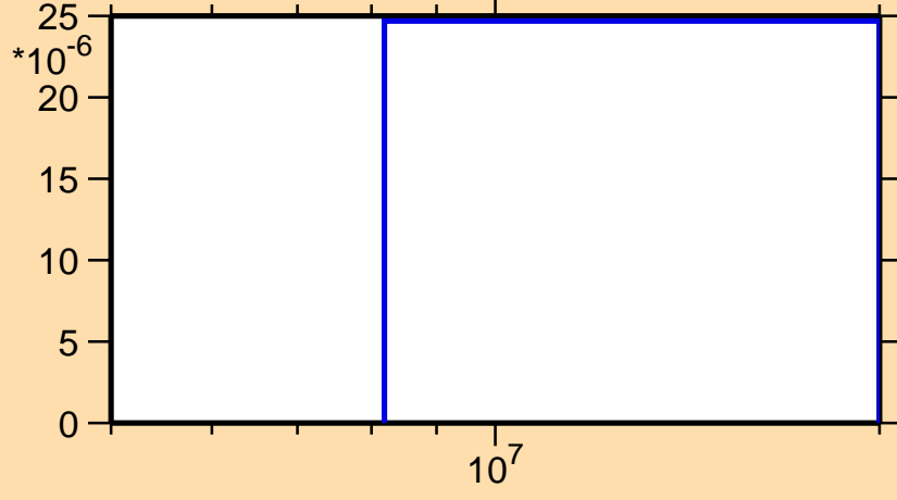
\sigma vs. E for ^{163}\text{Eu}(n,d)
