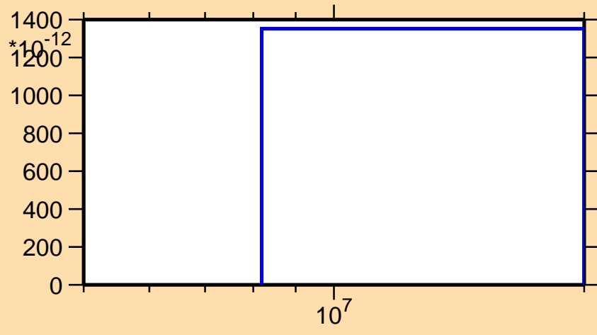
\sigma vs. E for ^{163}\text{Eu}(n,nd)
