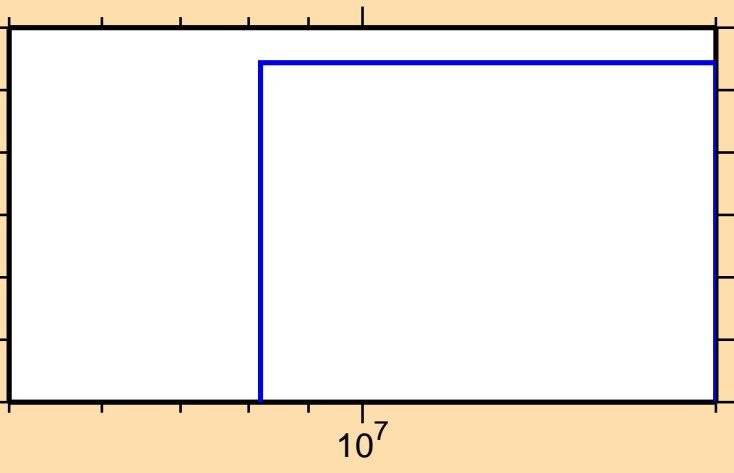
\sigma vs. E for ^{163}\text{Eu}(n,nt)
