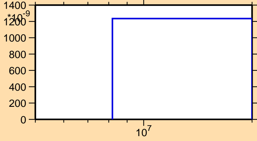
\sigma vs. E for ^{163}\text{Eu}(n,n\alpha)
