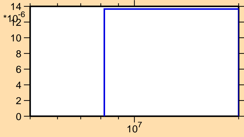
\sigma vs. E for ^{163}\text{Eu}(n,np)
