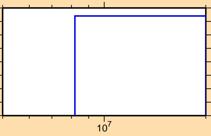
\sigma vs. E for ^{163}\text{Eu}(n,2np)
