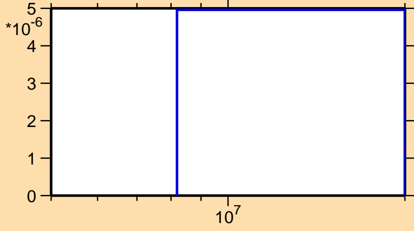
\sigma vs. E for ^{163}\text{Eu}(n,t)
