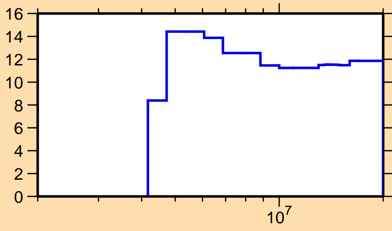
\Delta\sigma/\sigma vs. E for ^{164}\text{Eu}(n,\text{nonel.})
