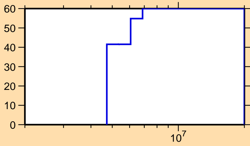
\Delta\sigma/\sigma vs. E for ^{164}\text{Eu}(n,\text{inel.})
