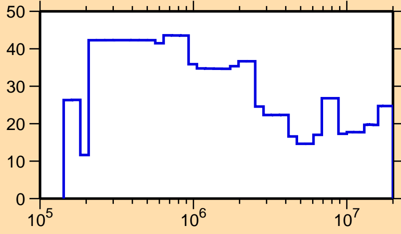
\Delta\sigma/\sigma vs. E for ^{164}\text{Eu}(n,\text{el.})
