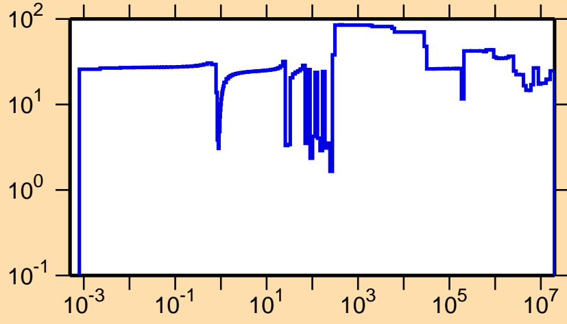
\Delta\sigma/\sigma vs. E for ^{164}\text{Eu}(n,\text{el.})
