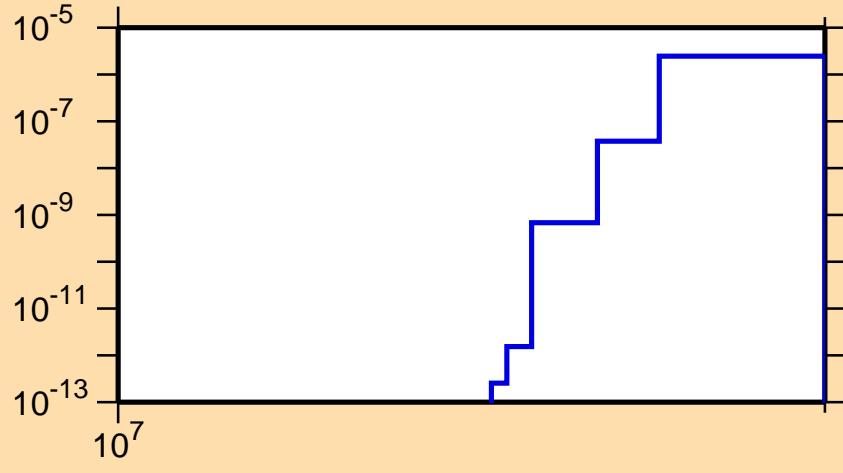
\sigma vs. E for ^{164}\text{Eu}(n,nt)
