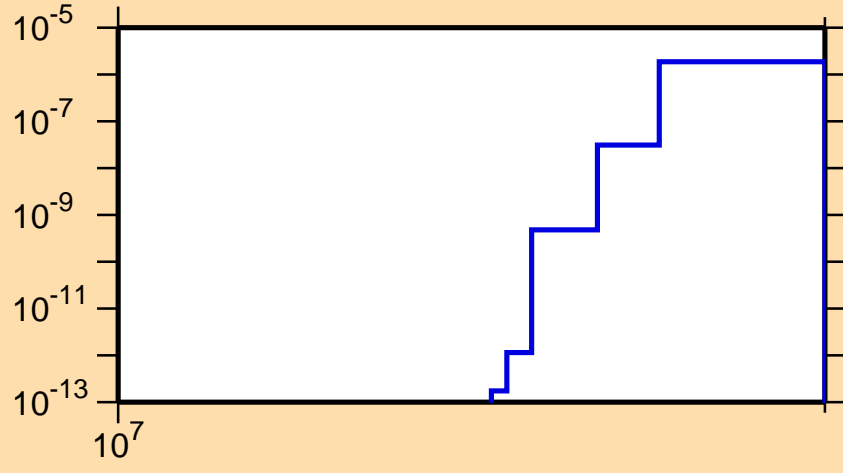
\sigma vs. E for ^{164}\text{Eu}(n,nd)
