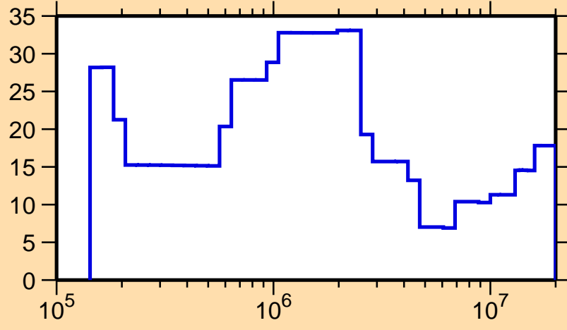
\Delta\sigma/\sigma vs. E for ^{164}\text{Eu}(n,\text{tot.})
