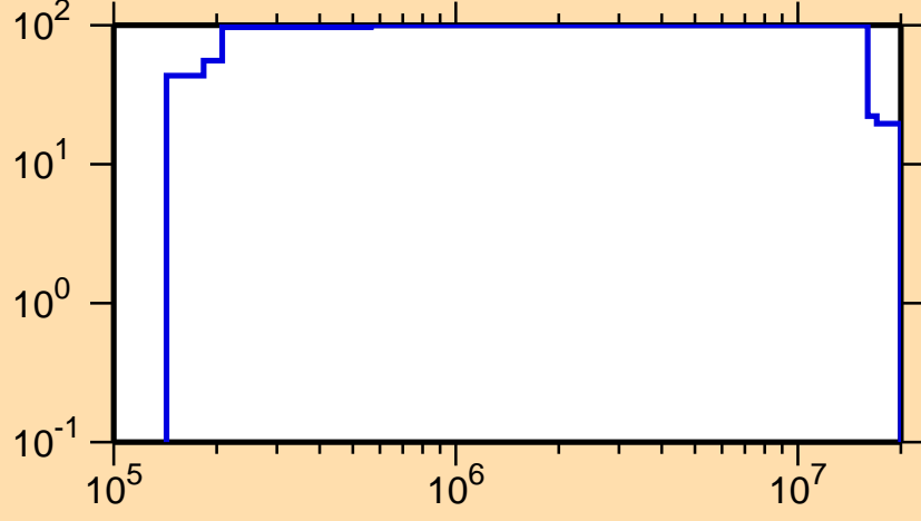
\Delta\sigma/\sigma vs. E for ^{164}\text{Eu}(n,n_1)
