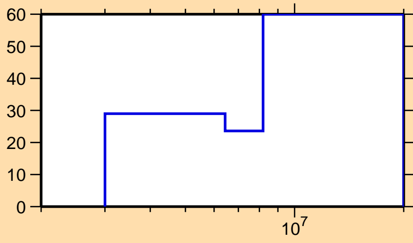
\Delta\sigma/\sigma vs. E for ^{164}\text{Eu}(n,2n)
