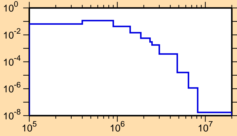
\sigma vs. E for ^{164}\text{Eu}(n,n_1)
