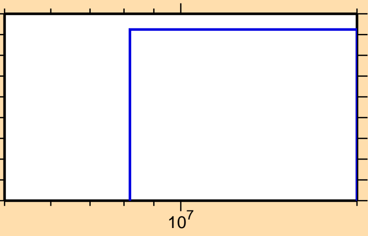
\sigma vs. E for ^{164}\text{Eu}(n,nd)
