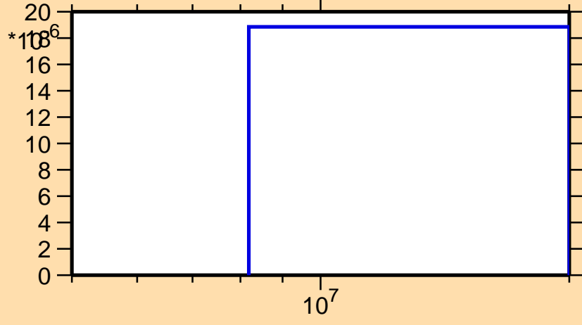
\sigma vs. E for ^{164}\text{Eu}(n,d)
