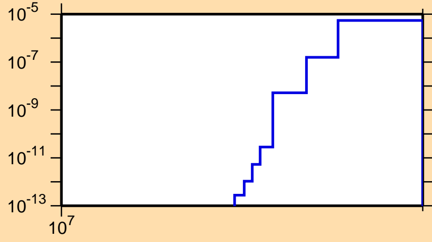
\sigma vs. E for ^{165}\text{Eu}(n,nt)
