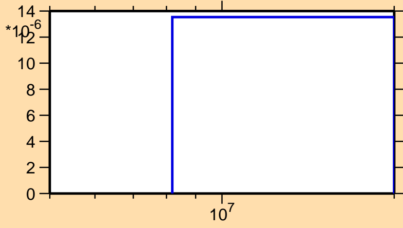
\sigma vs. E for ^{165}\text{Eu}(n,d)
