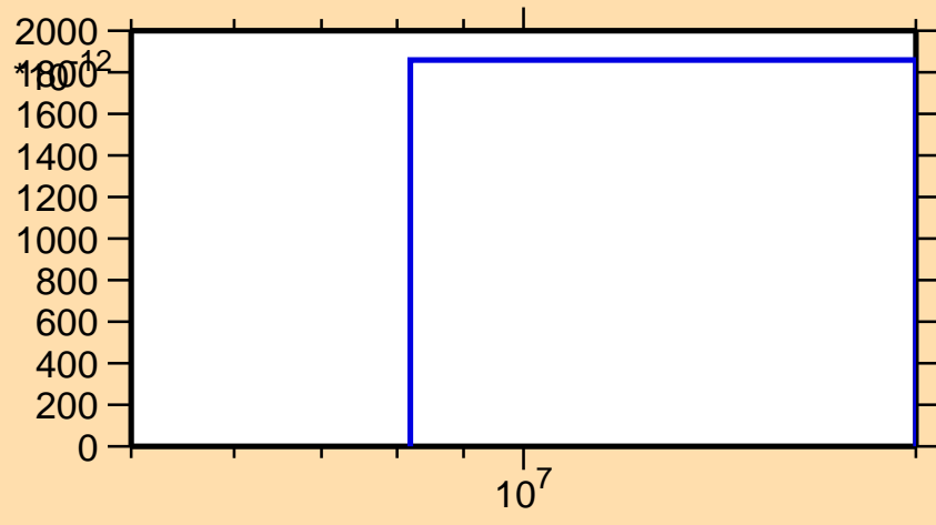
\sigma vs. E for ^{165}\text{Eu}(n,nd)
