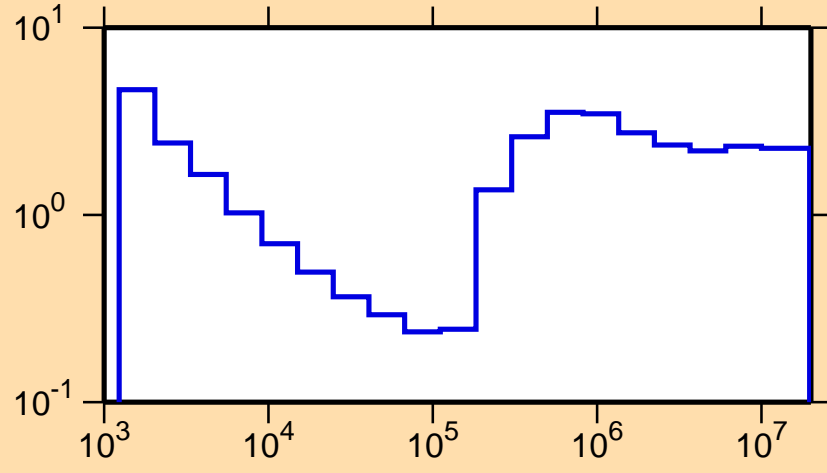
\sigma vs. E for ^{166}\text{Eu}(n,\text{nonel.})
