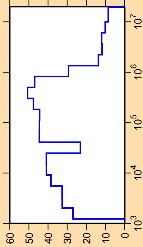
\Delta\sigma/\sigma vs. E for ^{166}\text{Eu}(n,\text{nonel.})
