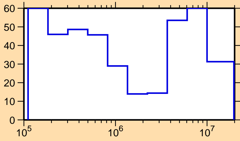
\Delta\sigma/\sigma vs. E for ^{166}\text{Eu}(n,n\text{cont.})
