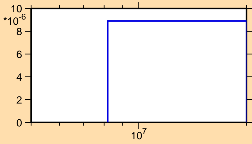
\sigma vs. E for ^{166}\text{Eu}(n,t)
