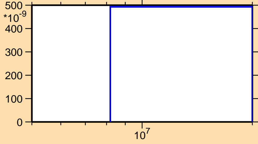
\sigma vs. E for ^{166}\text{Eu}(n,n\alpha)
