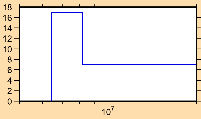
\Delta\sigma/\sigma vs. E for ^{166}\text{Eu}(n,el.)
