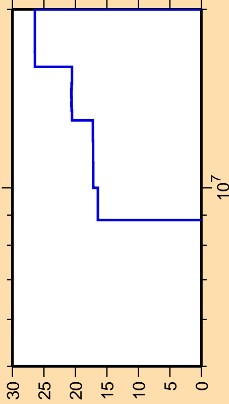
\Delta\sigma/\sigma vs. E for ^{18}\text{F}(n,\alpha)
