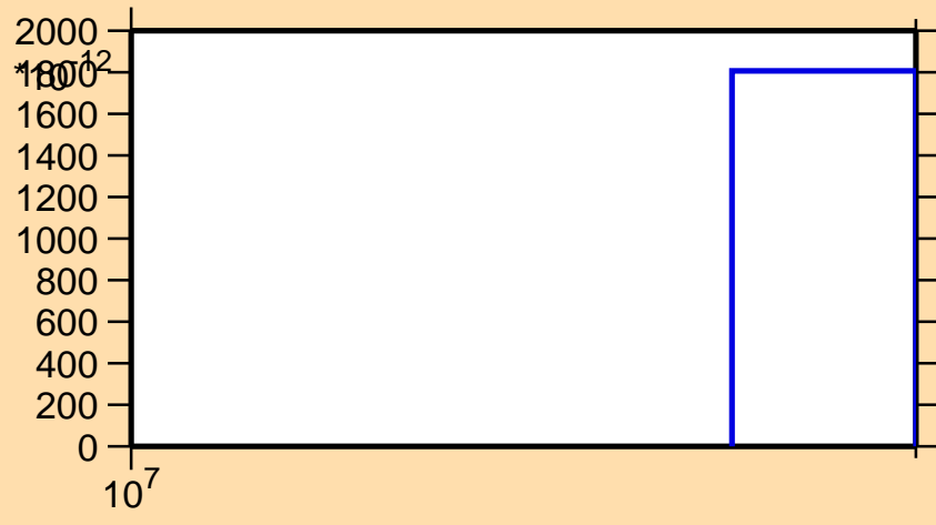
\sigma vs. E for ^{18}\text{F}(n,\text{pd})
