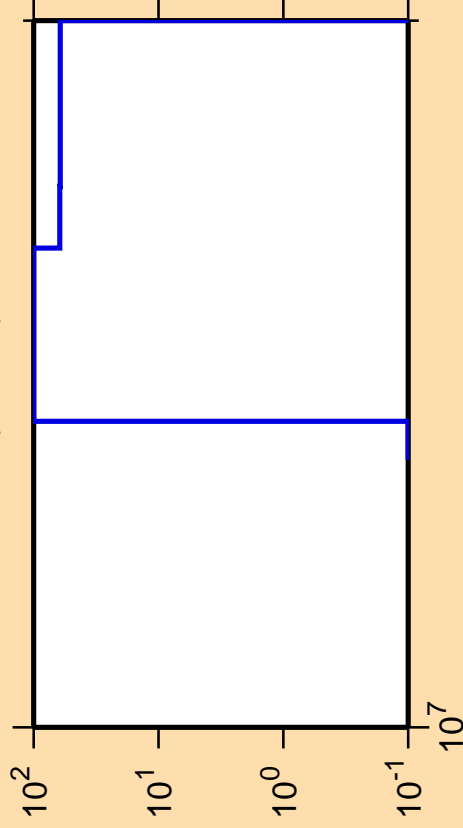
\Delta\sigma/\sigma vs. E for ^{18}\text{F} (mt 45)
