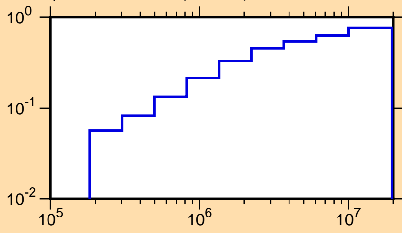
\mu vs. E for ^{18}\text{F} (mt251)
