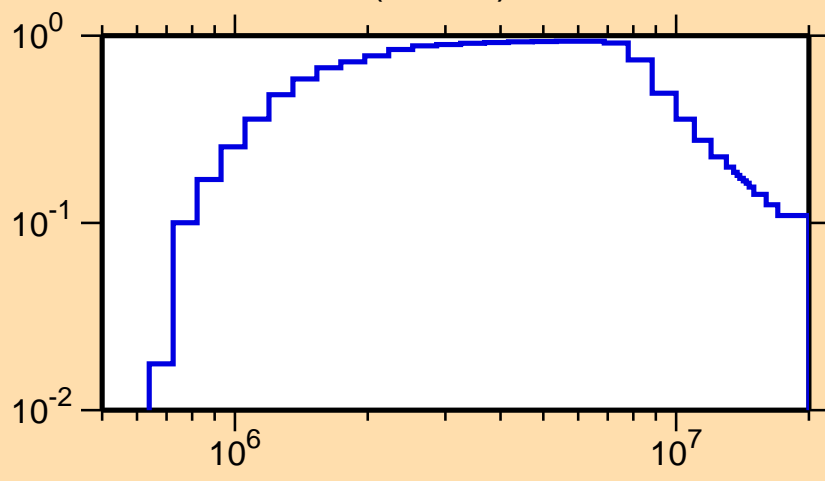
\sigma vs. E for ^{20}\text{F}(n,\text{inel.})
