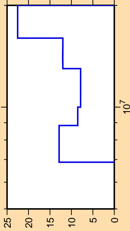
\Delta\sigma/\sigma vs. E for ^{20}\text{F}(n,2n)
