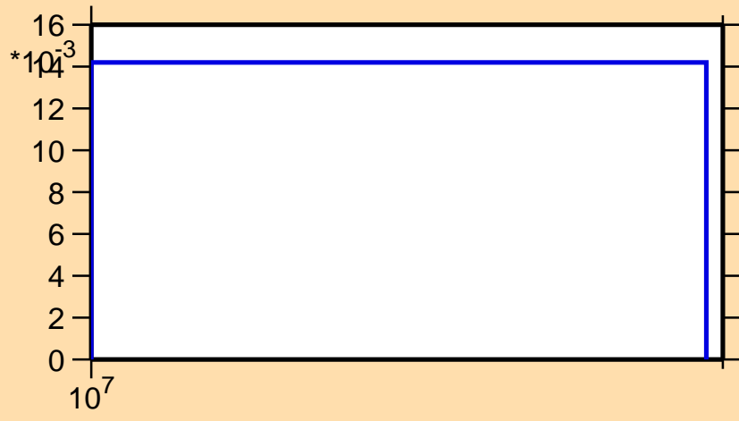
\sigma vs. E for ^{20}\text{F}(n,2n\alpha)
