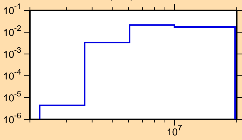
\sigma vs. E for ^{20}\text{F}(n,\alpha)
