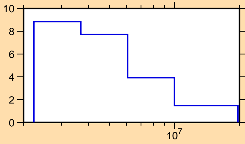
\Delta\sigma/\sigma vs. E for ^{20}\text{F}(n,\text{tot.})
