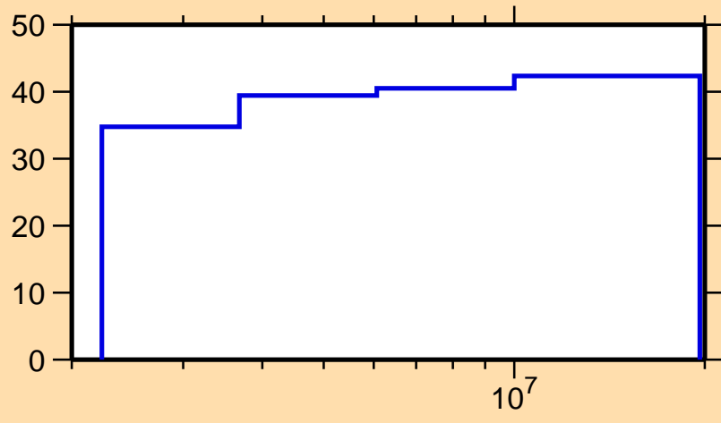
\Delta\sigma/\sigma vs. E for ^{20}\text{F}(n,p)
