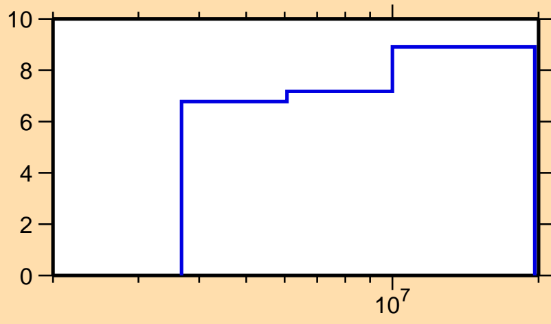
\Delta\sigma/\sigma vs. E for ^{20}\text{F}(n,\text{nonel.})
