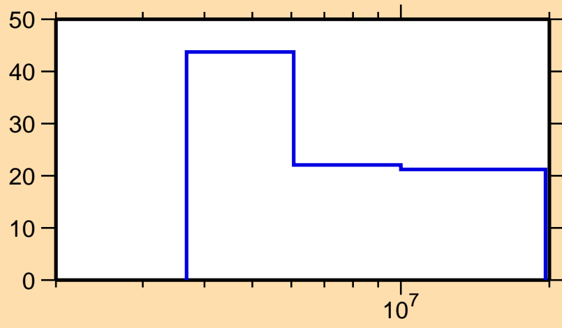
\Delta\sigma/\sigma vs. E for ^{20}\text{F}(n,ncont.)
