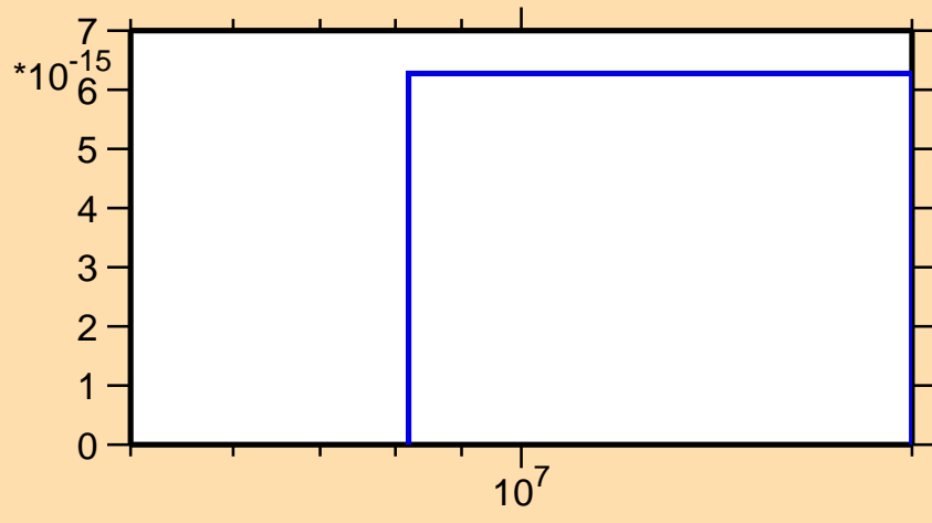
\sigma vs. E for ^{20}\text{F}(\text{mt117})
