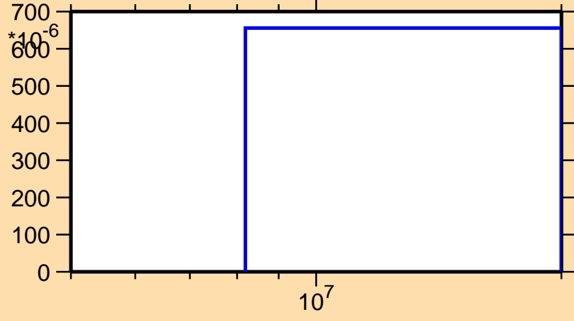
\sigma vs. E for ^{20}\text{F}(n,\text{nd})
