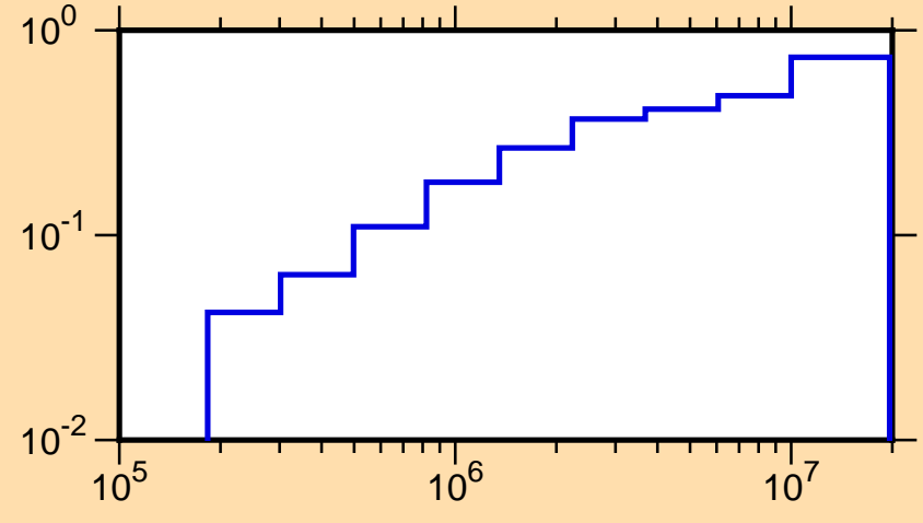
\mu vs. E for ^{21}\text{F} (mt251)
