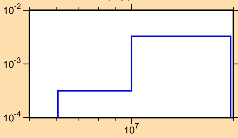
\sigma vs. E for ^{21}\text{F}(n,p)
