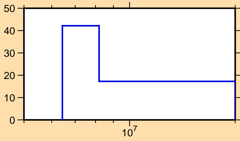
\Delta\sigma/\sigma vs. E for ^{21}\text{F}(n,n\text{cont.})
