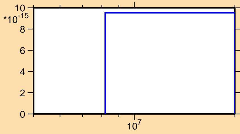
\sigma vs. E for ^{21}\text{F}(n,2np)
