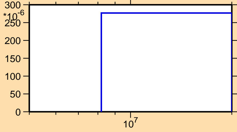
\sigma vs. E for ^{21}\text{F}(n,3n)
