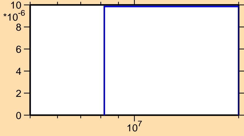
\sigma vs. E for ^{21}\text{F}(n,nt)
