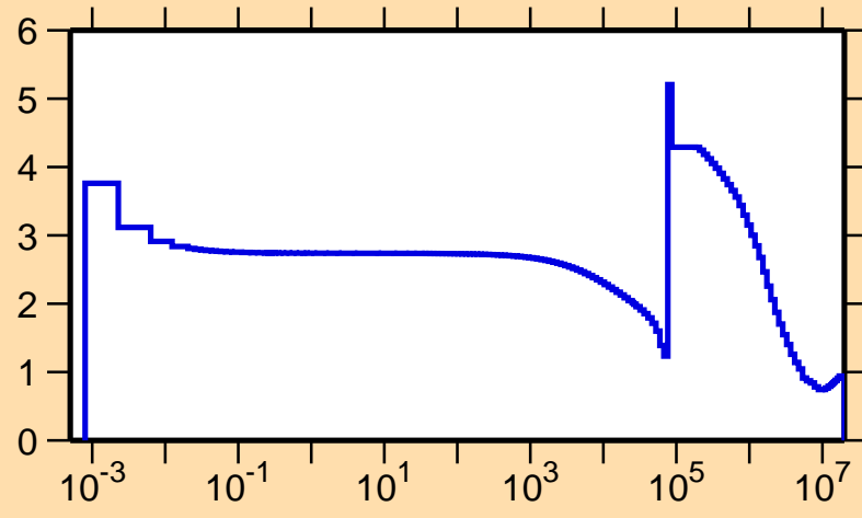
\sigma vs. E for ^{22}\text{F}(n,\text{el.})
