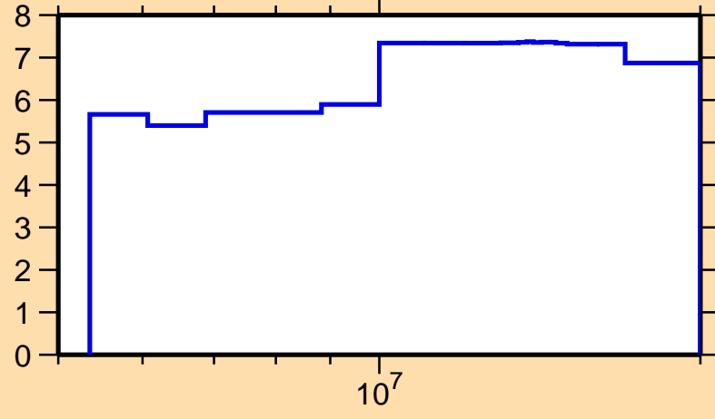
\Delta\sigma/\sigma vs. E for ^{22}\text{F}(n,el.)
