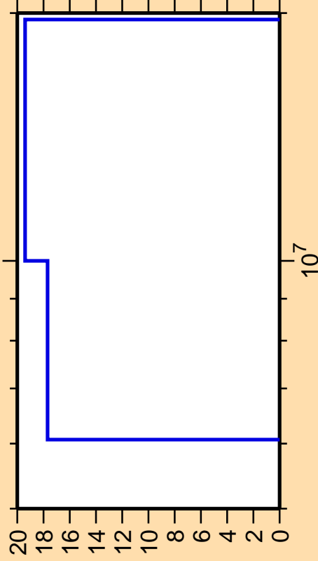
\Delta\sigma/\sigma vs. E for ^{22}\text{F}(n,2n)
