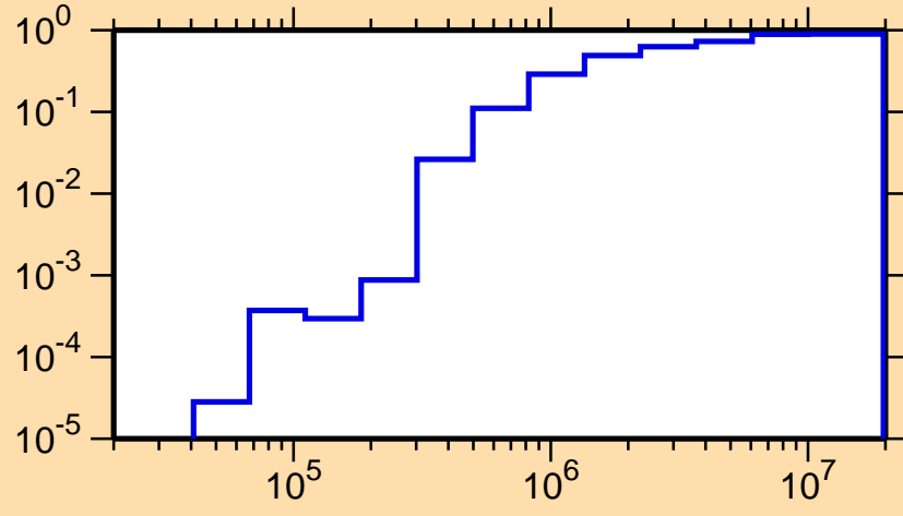
\sigma vs. E for ^{22}\text{F}(n,\text{nonel.})
