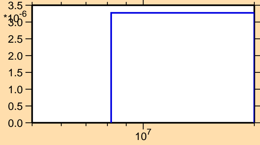
\sigma vs. E for ^{22}\text{F}(n,\text{nd})
