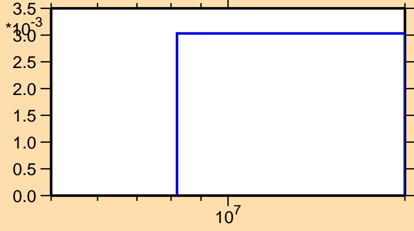
\sigma vs. E for ^{22}\text{F}(n,3n)
