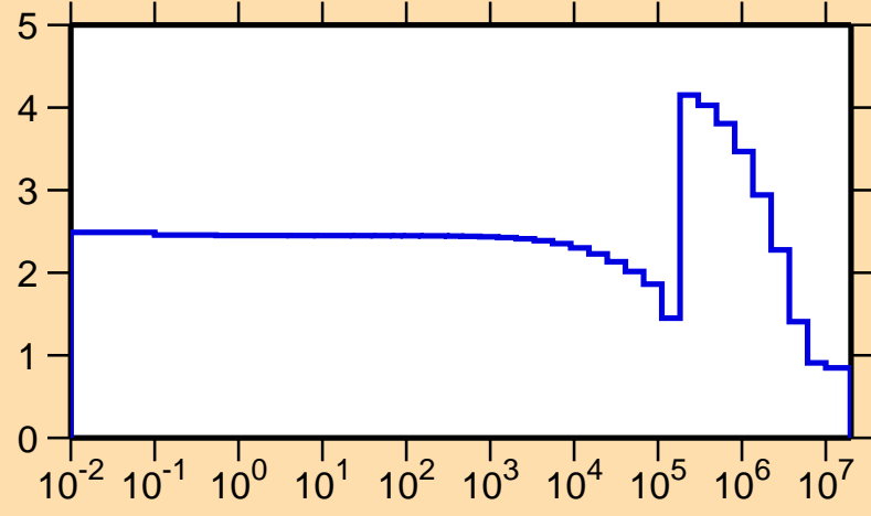
\sigma vs. E for ^{23}\text{F}(n,\text{el.})
