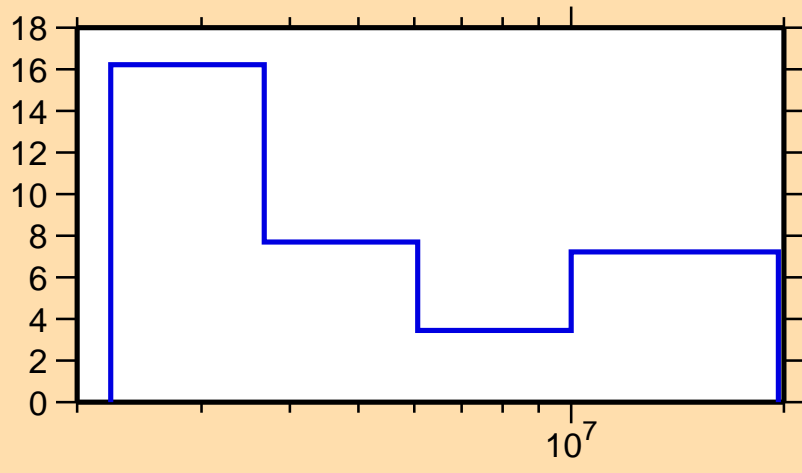
\Delta\sigma/\sigma vs. E for ^{23}\text{F}(n,\text{nonel.})
