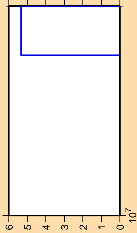
\Delta\sigma/\sigma vs. E for ^{52}\text{Fe}(n,\text{pt})
