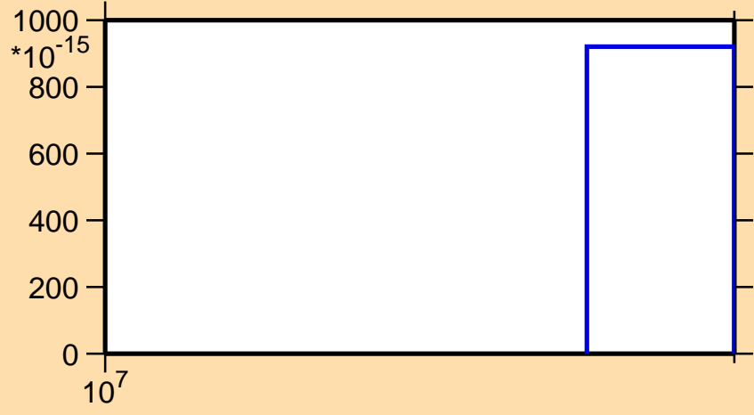
\sigma vs. E for ^{52}\text{Fe}(n,\text{pt})
