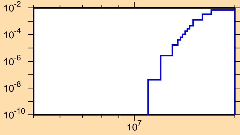
\sigma vs. E for ^{52}\text{Fe}(n,n\alpha)
