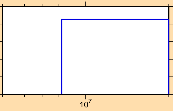
\sigma vs. E for ^{52}\text{Fe}(n,p\alpha)
