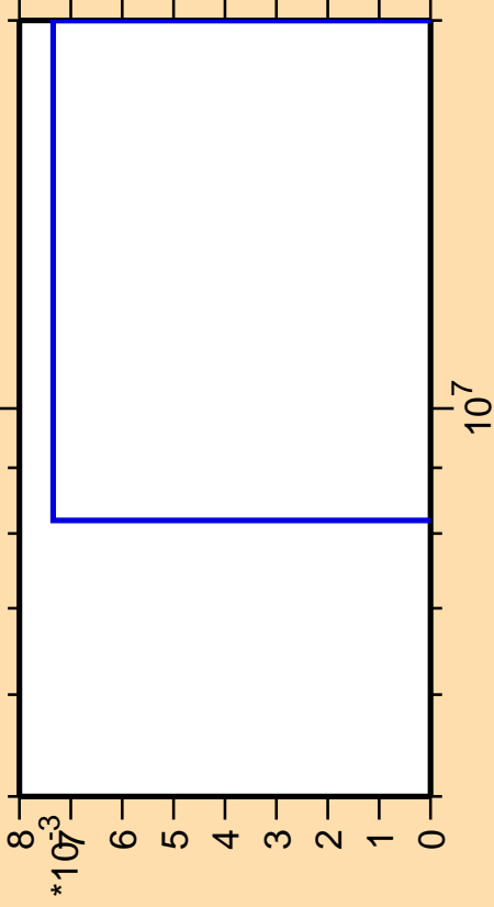
\Delta\sigma/\sigma vs. E for ^{52}\text{Fe}(\text{mt117})
