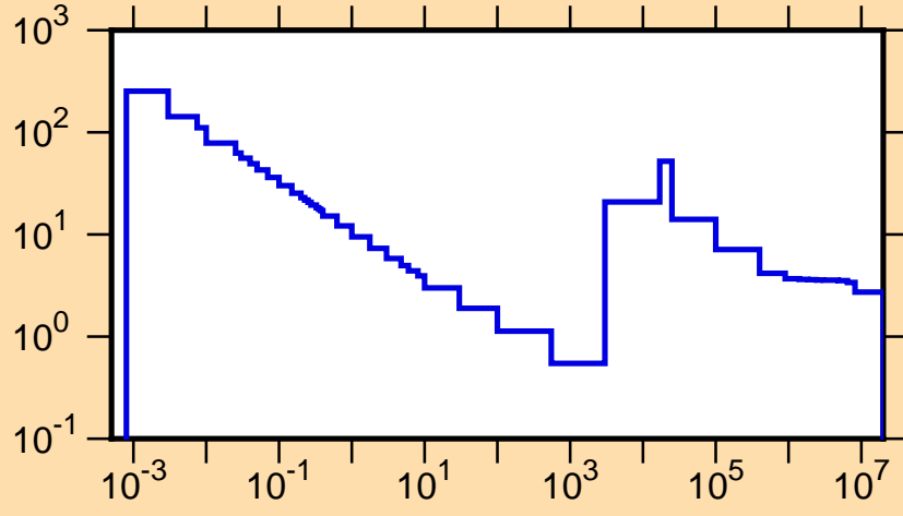
\sigma vs. E for ^{52}\text{Fe}(n,\text{tot.})
