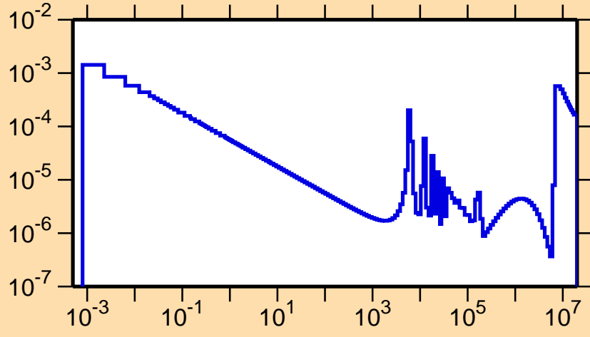
\sigma vs. E for ^{52}\text{Fe}(n,\gamma)
