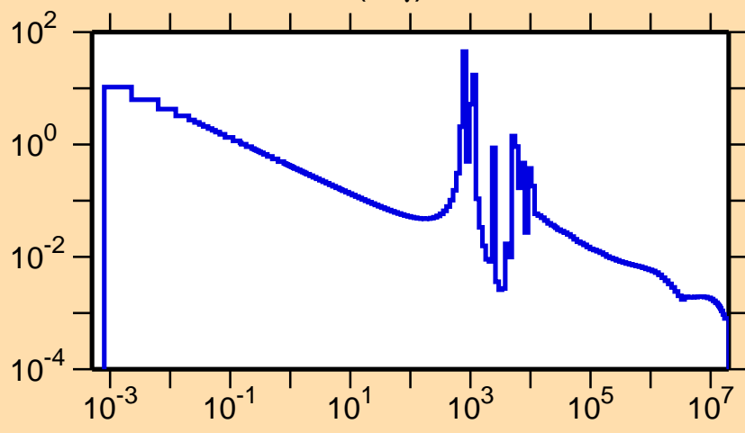
\sigma vs. E for ^{53}\text{Fe}(n,\gamma)
