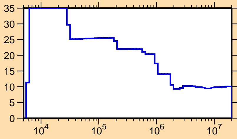
\Delta\sigma/\sigma vs. E for ^{53}\text{Fe}(n,\text{nonel.})
