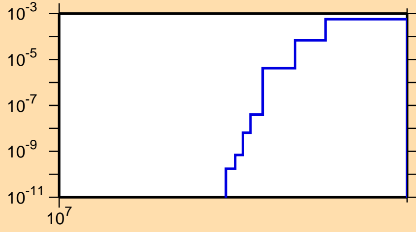
\sigma vs. E for ^{53}\text{Fe}(n,pd)
