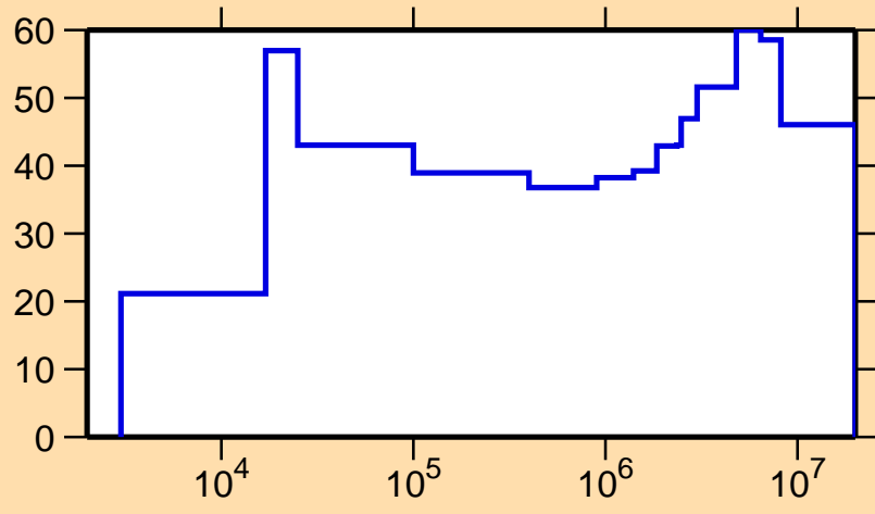
\Delta\sigma/\sigma vs. E for ^{53}\text{Fe}(n,\gamma)
