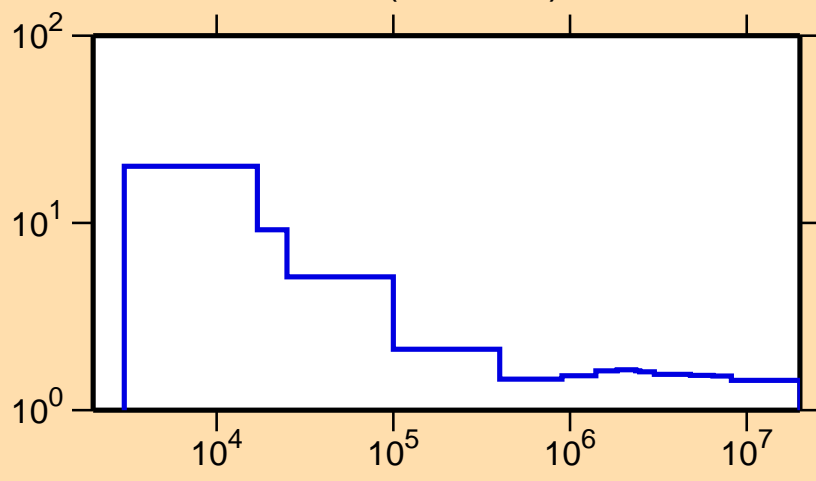
\sigma vs. E for ^{53}\text{Fe}(n,\text{nonel.})
