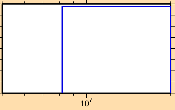
\sigma vs. E for ^{53}\text{Fe}(n,\text{pd})
