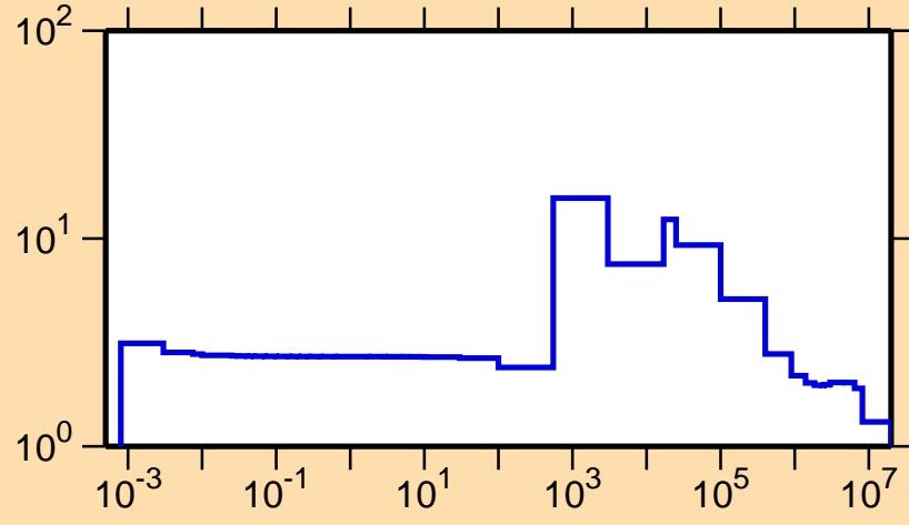
\sigma vs. E for ^{53}\text{Fe}(n,\text{el.})
