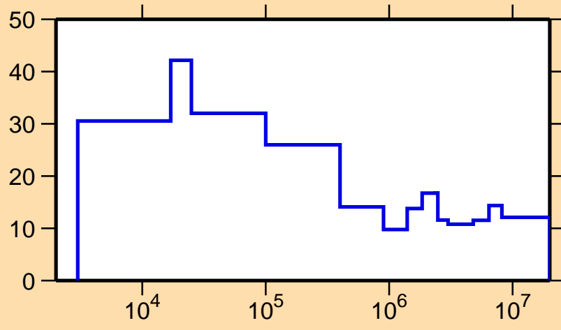
\Delta\sigma/\sigma vs. E for ^{53}\text{Fe}(n,el.)
