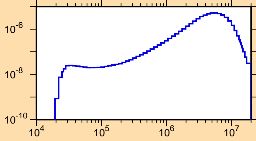
\sigma vs. E for ^{53}\text{Fe}(n,n_3)
