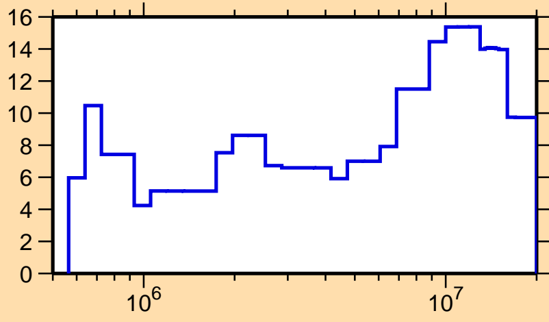
\Delta\sigma/\sigma vs. E for ^{54}\text{Fe}(n,el.)
