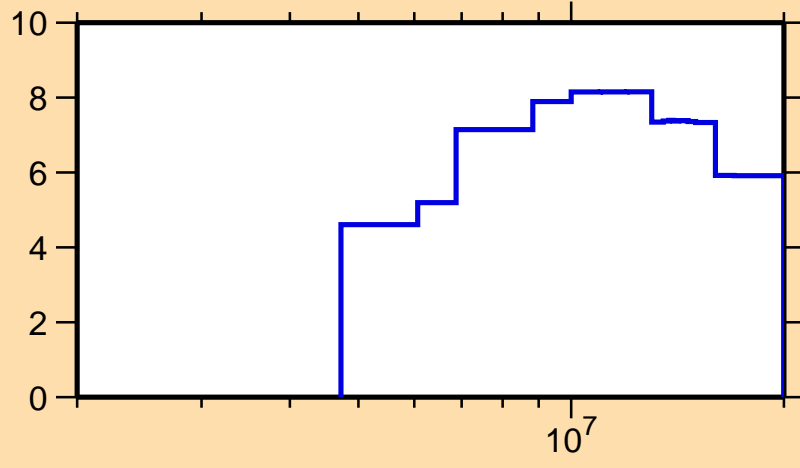
\Delta\sigma/\sigma vs. E for ^{54}\text{Fe}(n,\text{tot.})
