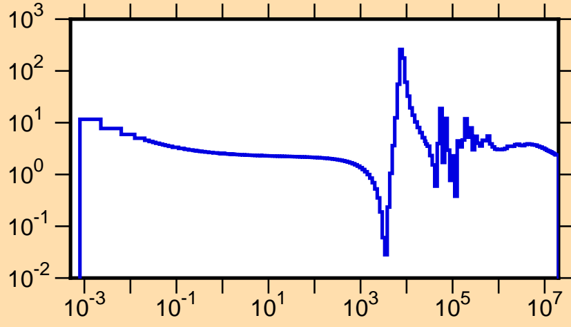
\sigma vs. E for ^{54}\text{Fe}(n,\text{tot.})
