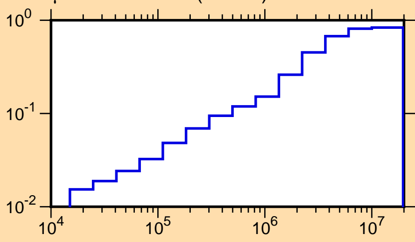
\mu vs. E for ^{54}\text{Fe}(\text{mt251})
