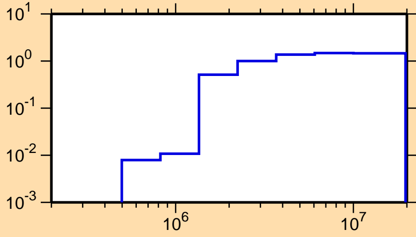
\sigma vs. E for ^{54}\text{Fe}(n,\text{nonel.})
