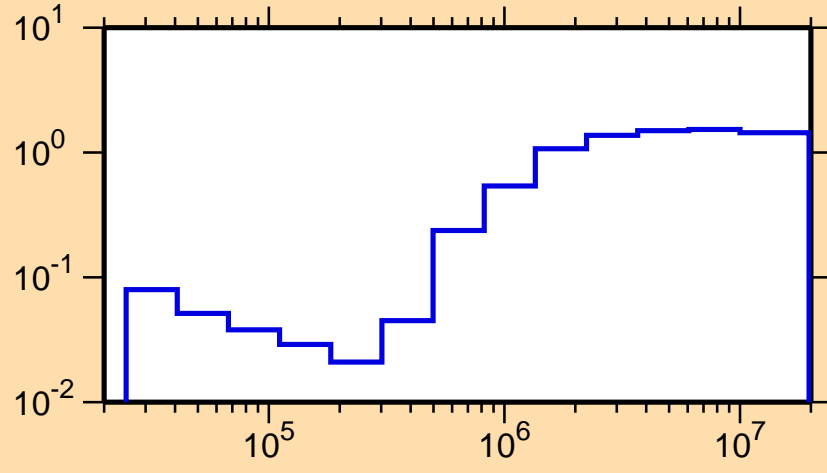
\sigma vs. E for ^{55}\text{Fe}(n,\text{nonel.})
