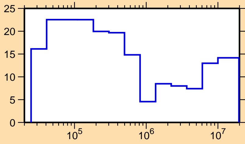
\Delta\sigma/\sigma vs. E for ^{55}\text{Fe}(n,el.)
