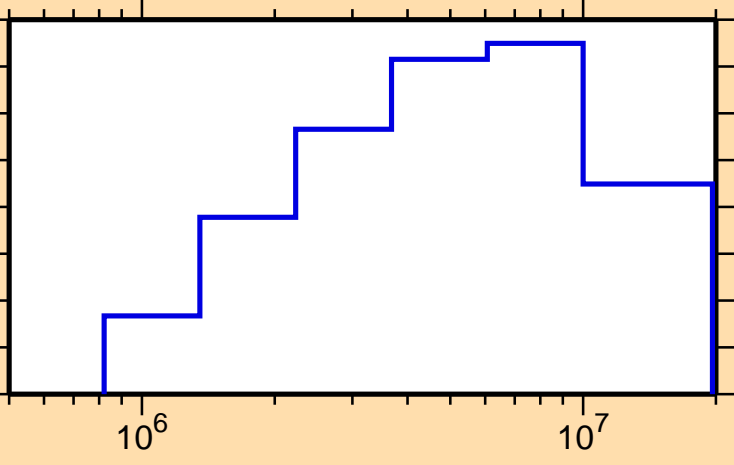
\sigma vs. E for ^{56}\text{Fe}(n,\text{inel.})
