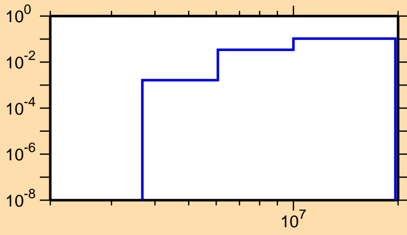
\sigma vs. E for ^{56}\text{Fe}(n,p)
