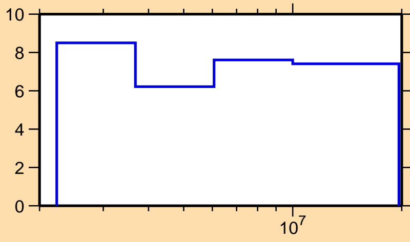
\Delta\sigma/\sigma vs. E for ^{56}\text{Fe}(n,el.)
