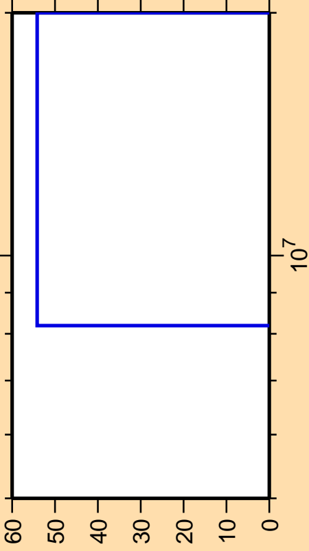
\Delta\sigma/\sigma vs. E for ^{56}\text{Fe}(n,\gamma)
