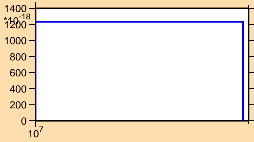
\sigma vs. E for ^{58}\text{Fe}(n,p\alpha)
