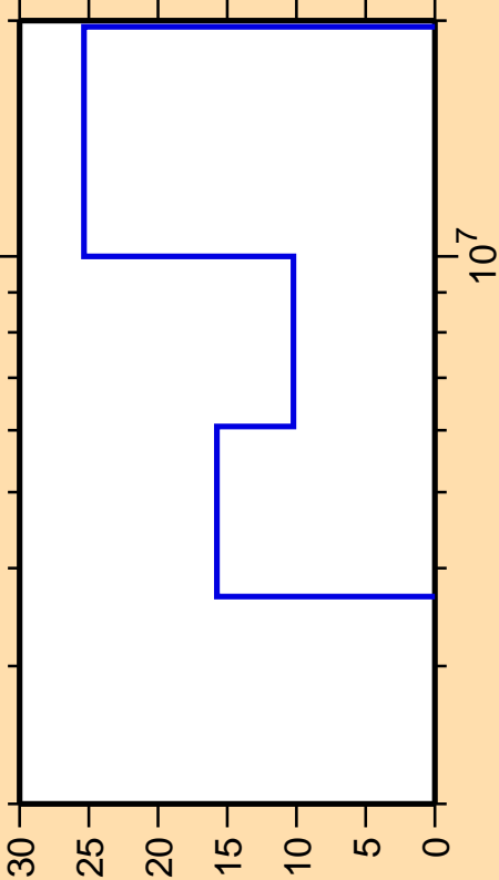
\Delta\sigma/\sigma vs. E for ^{58}\text{Fe}(n,n\text{cont.})
