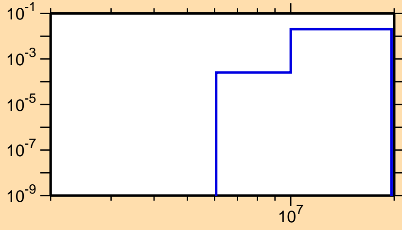
\sigma vs. E for ^{58}\text{Fe}(n,p)
