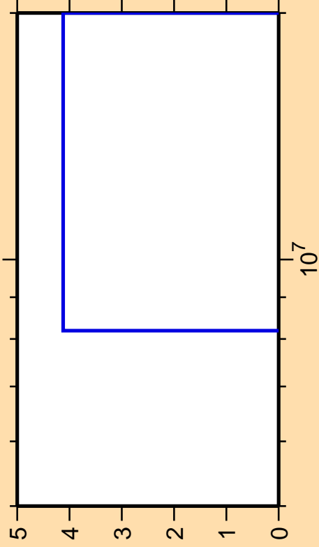
\Delta\sigma/\sigma vs. E for ^{58}\text{Fe}(n,\text{He}3)
