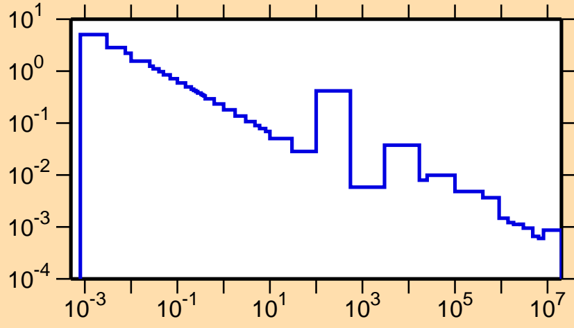
\sigma vs. E for ^{58}\text{Fe}(n,\gamma)
