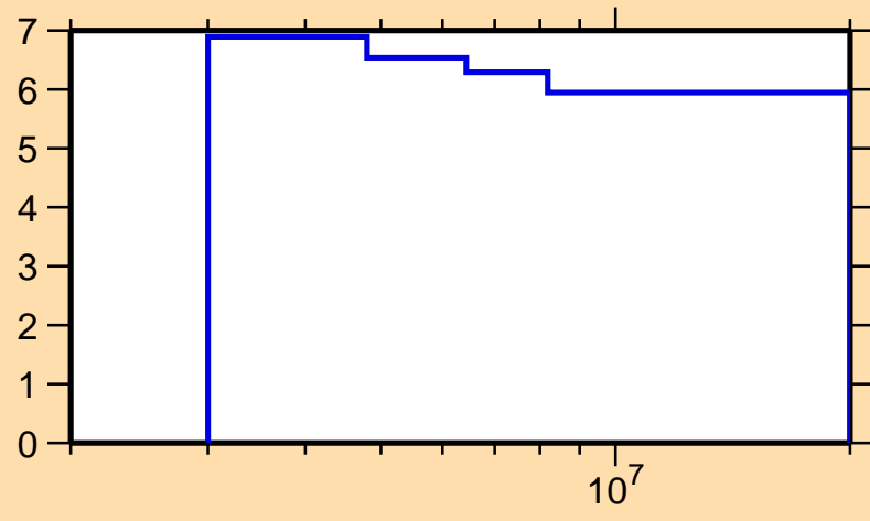
\Delta\sigma/\sigma vs. E for ^{58}\text{Fe}(n,n_{\text{nonel}})
