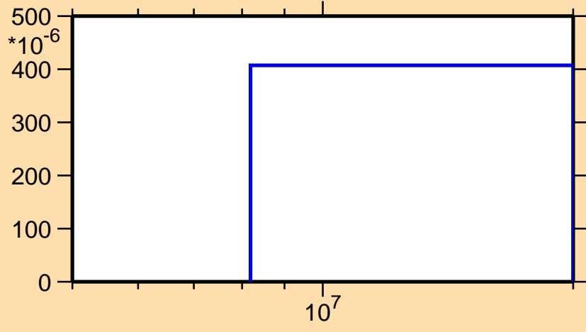
\sigma vs. E for ^{58}\text{Fe}(n,d)
