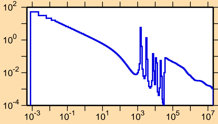
\sigma vs. E for ^{59}\text{Fe}(n,\gamma)
