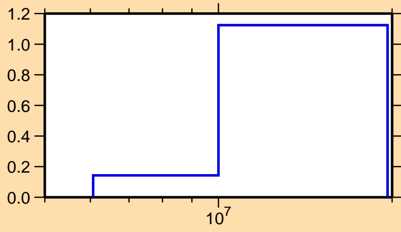
\sigma vs. E for ^{59}\text{Fe}(n,2n)
