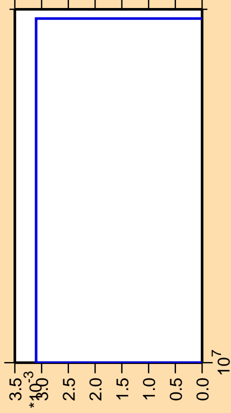
\Delta\sigma/\sigma vs. E for ^{59}\text{Fe}(n,p\alpha)
