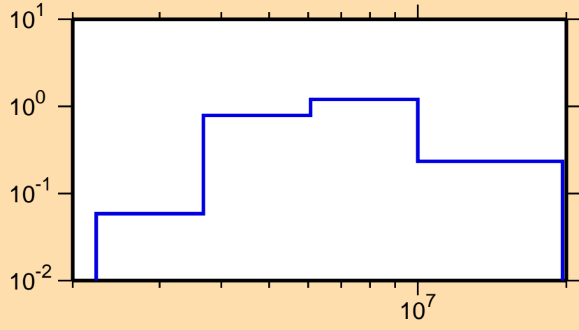
\sigma vs. E for ^{59}\text{Fe}(n,n\text{cont.})
