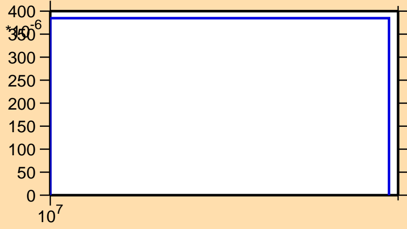
\sigma vs. E for ^{59}\text{Fe}(n,d)
