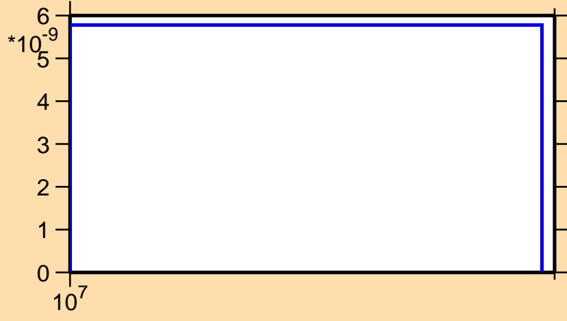
\sigma vs. E for ^{59}\text{Fe}(n,\text{nd})
