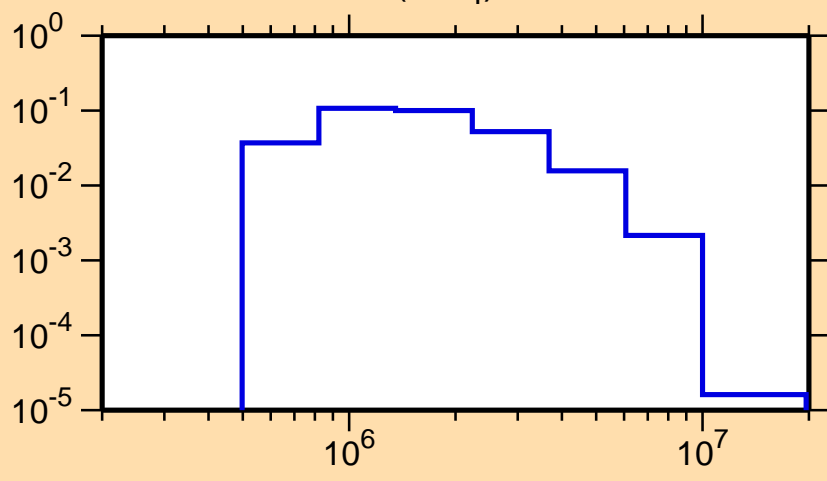
\sigma vs. E for ^{59}\text{Fe}(n,n_4)
