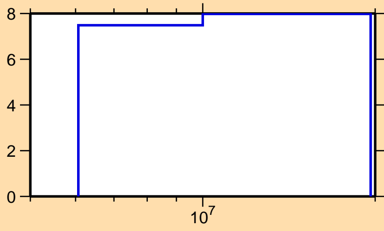
\Delta\sigma/\sigma vs. E for ^{59}\text{Fe}(n,\text{nonel.})
