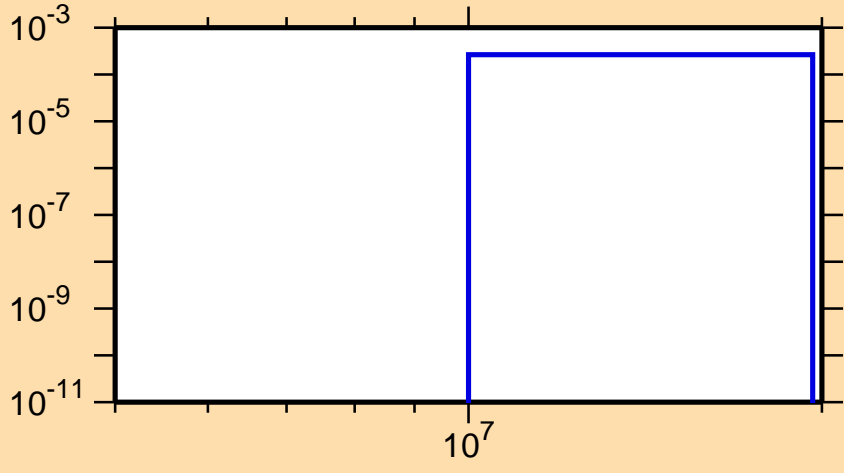
\sigma vs. E for ^{59}\text{Fe}(n,\alpha)
