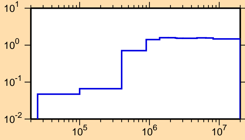
\sigma vs. E for ^{59}\text{Fe}(n,\text{nonel.})
