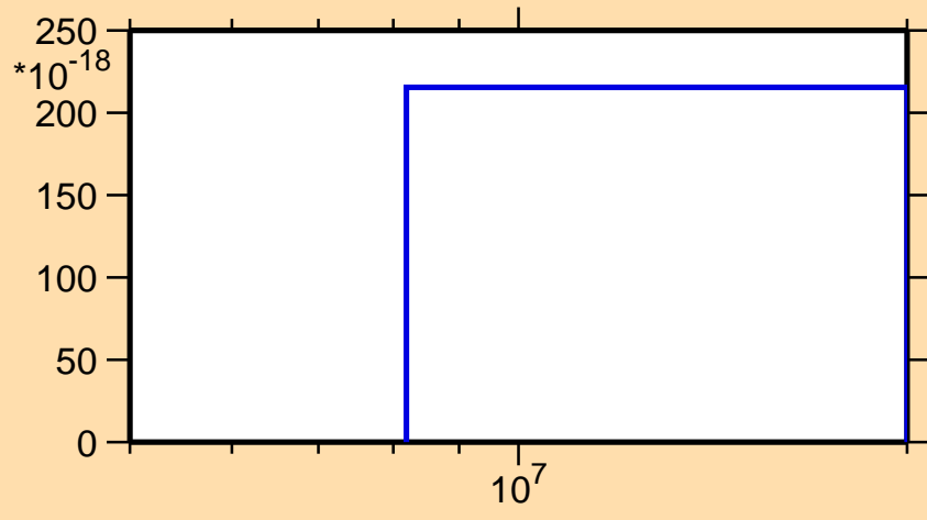
\sigma vs. E for ^{59}\text{Fe}(n,nt)
