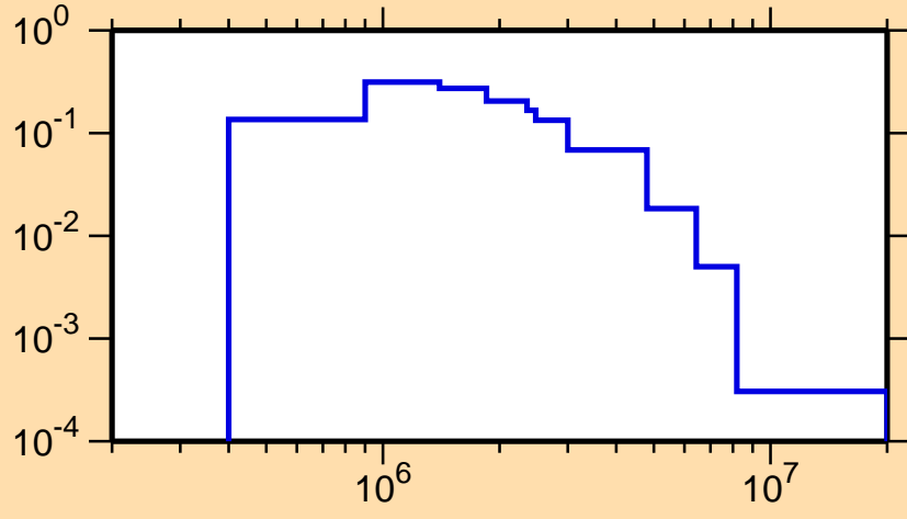
\sigma vs. E for ^{59}\text{Fe}(n,n_3)
