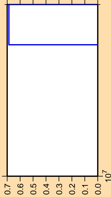
\Delta\sigma/\sigma vs. E for ^{60}\text{Fe}(n,\text{nd})
