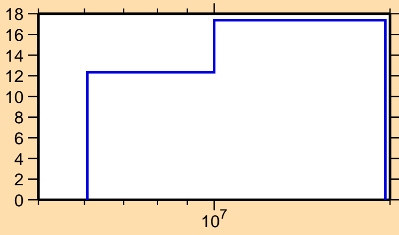
\Delta\sigma/\sigma vs. E for ^{60}\text{Fe}(n,el.)
