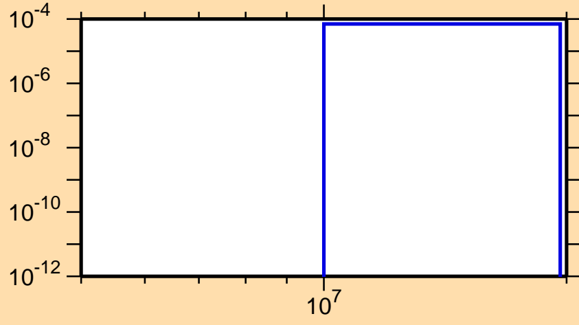
\sigma vs. E for ^{60}\text{Fe}(n,n\alpha)
