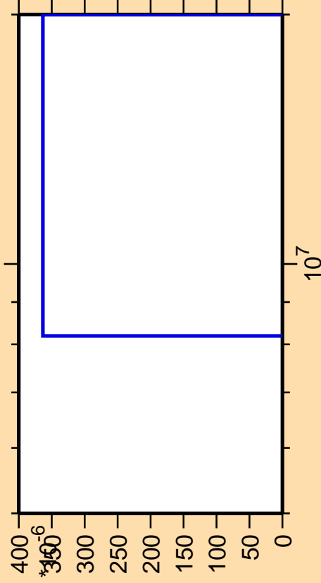
\Delta\sigma/\sigma vs. E for ^{60}\text{Fe}(n,2n\alpha)
