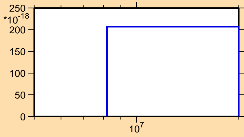
\sigma vs. E for ^{60}\text{Fe}(n,2n\alpha)
