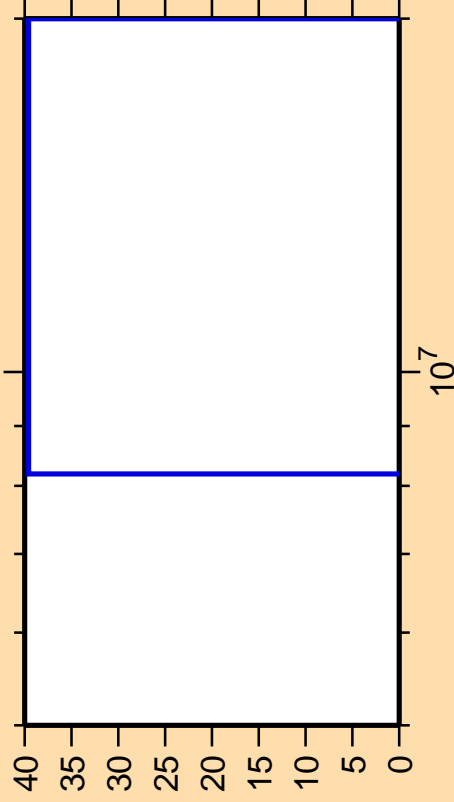
\Delta\sigma/\sigma vs. E for ^{60}\text{Fe}(n,p)
