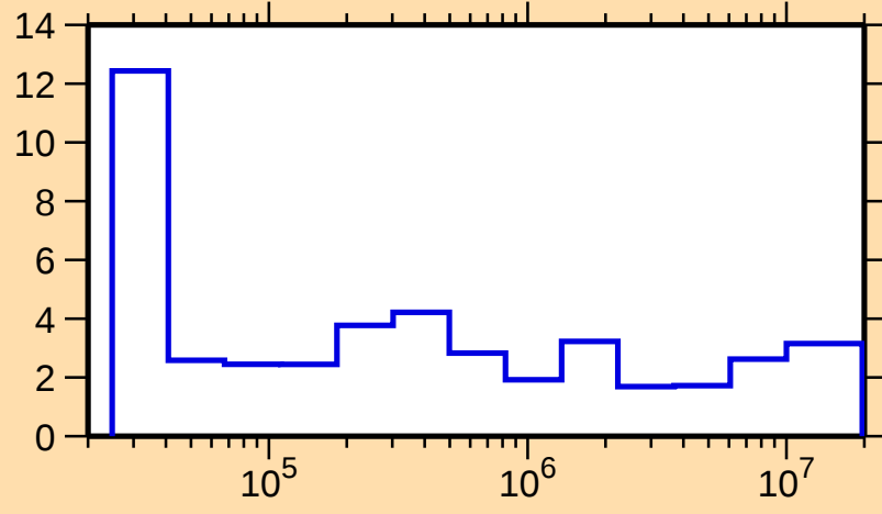
\Delta\sigma/\sigma vs. E for ^{61}\text{Fe}(n,\text{tot.})
