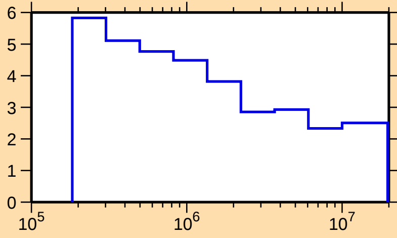
\Delta\sigma/\sigma vs. E for ^{61}\text{Fe}(\text{n,nonel.})
