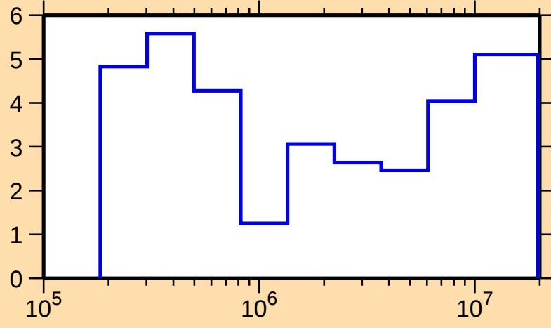
\Delta\sigma/\sigma vs. E for ^{61}\text{Fe}(\text{n,el.})
