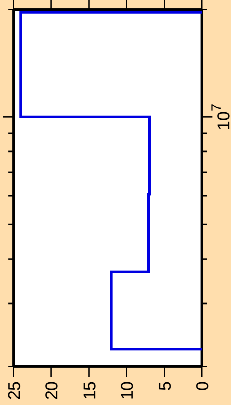
\Delta\sigma/\sigma vs. E for ^{61}\text{Fe}(n,\text{ncont.})
