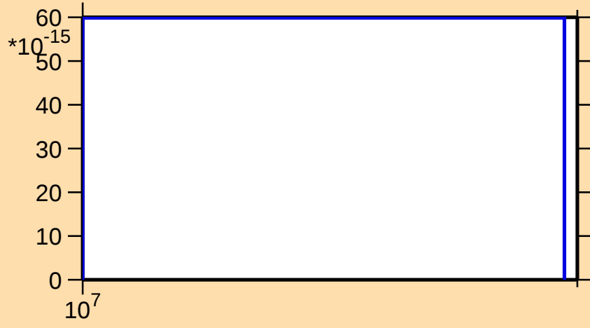
\sigma vs. E for ^{61}\text{Fe}(n,\text{nt})
