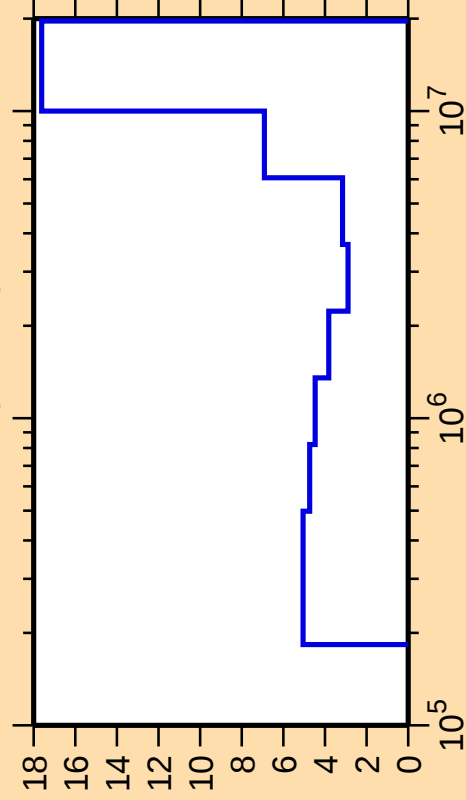
\Delta\sigma/\sigma vs. E for ^{61}\text{Fe}(\text{n,inel.})
