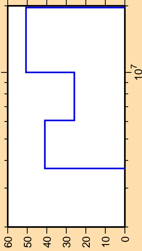
\Delta\sigma/\sigma vs. E for ^{62}\text{Fe}(n,n\text{cont.})
