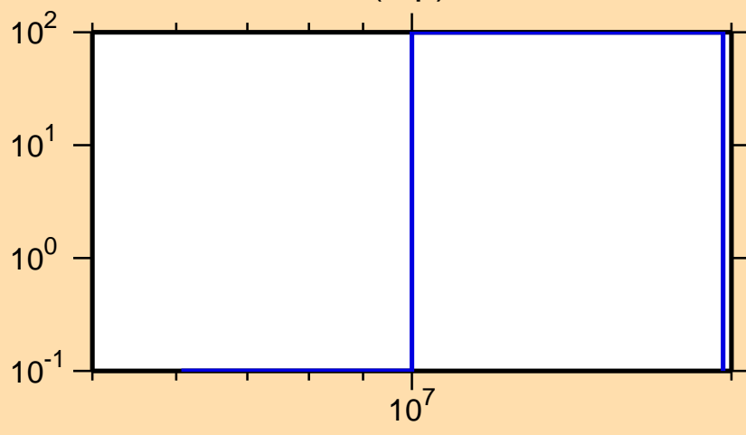
\Delta\sigma/\sigma vs. E for ^{62}\text{Fe}(n,p)
