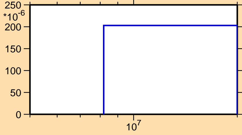
\sigma vs. E for ^{62}\text{Fe}(n,p)
