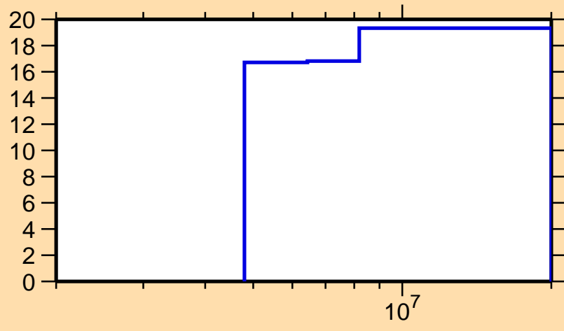
\Delta\sigma/\sigma vs. E for ^{62}\text{Fe}(n,n\text{onel.})
