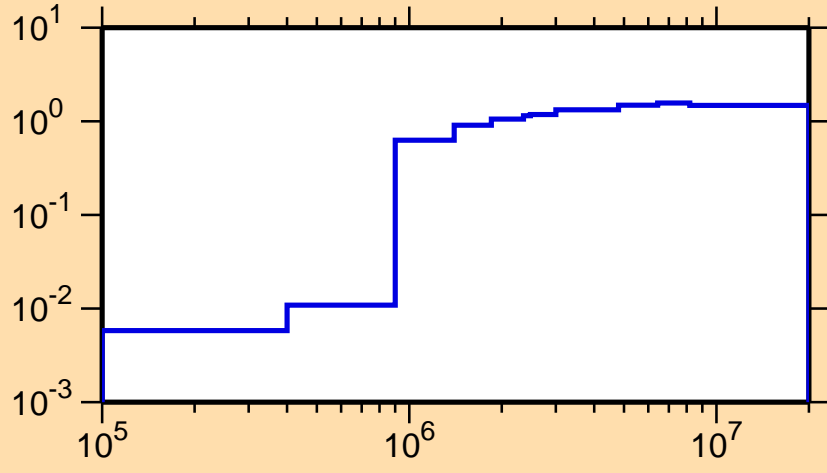
\sigma vs. E for ^{62}\text{Fe}(n,\text{nonel.})
